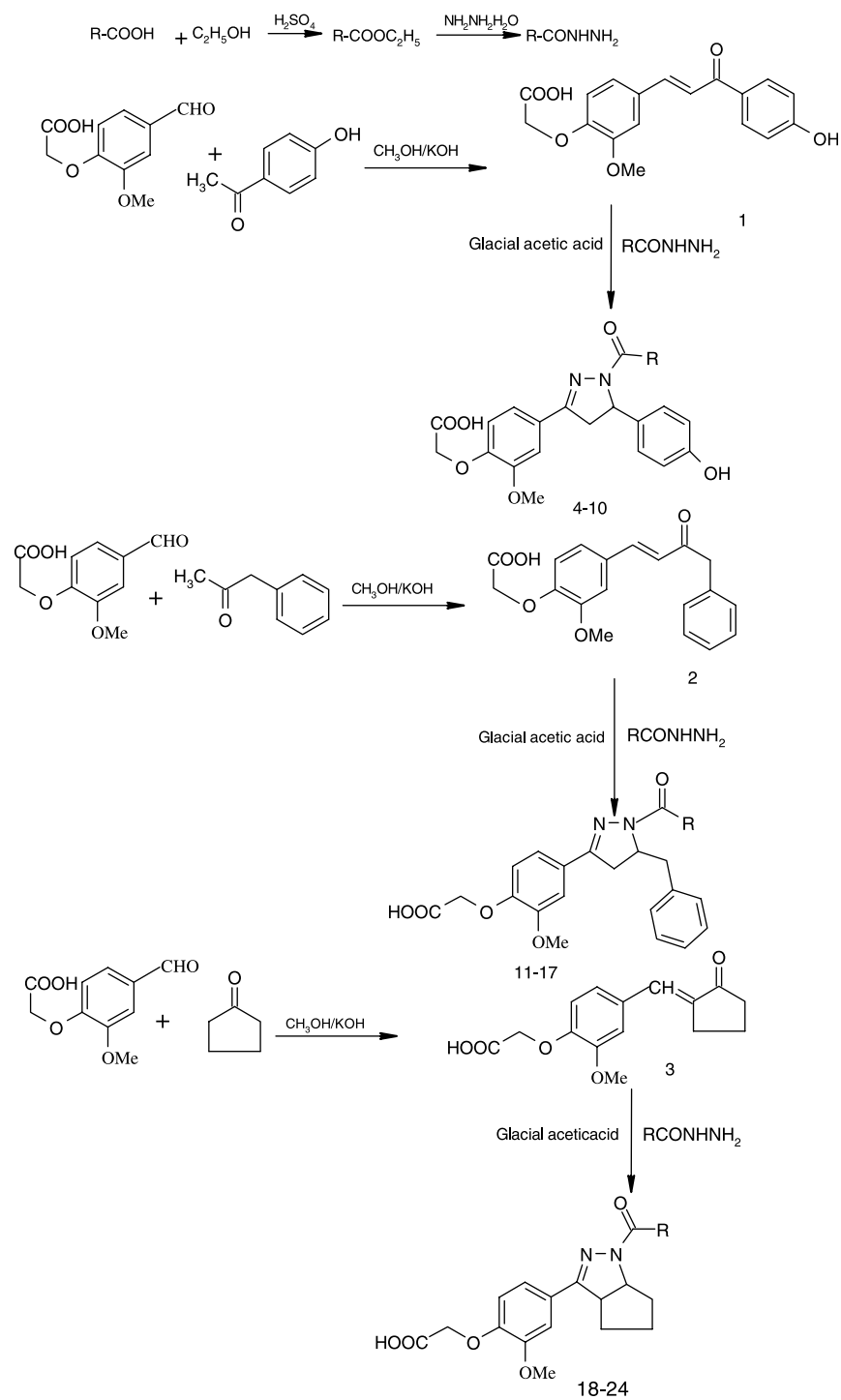
Scheme 1. Protocol for the synthesis of phenoxy acetic acid derivatives.
